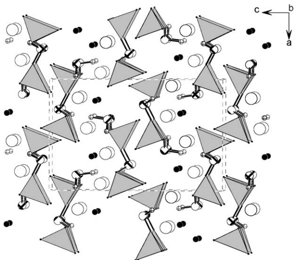
Fig. 3. View of the structure of BaZn(TeO_3)Cl_2 down the b -axis. ZnO_3Cl and ZnO_2Cl_2 tetrahedra are shaded in gray. Ba, Te, Cl and O atoms are represented by open (large), hatched, black and crossed circles, respectively.
